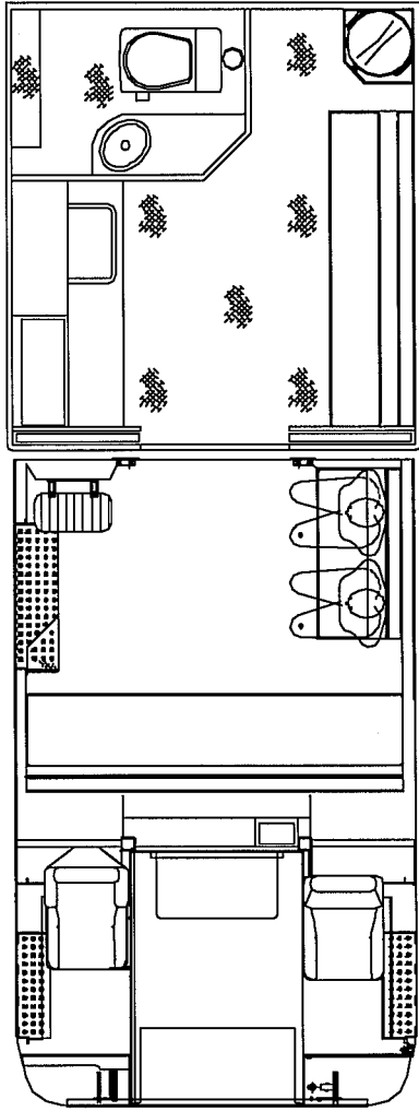
TOP VIEW INTERIOR
